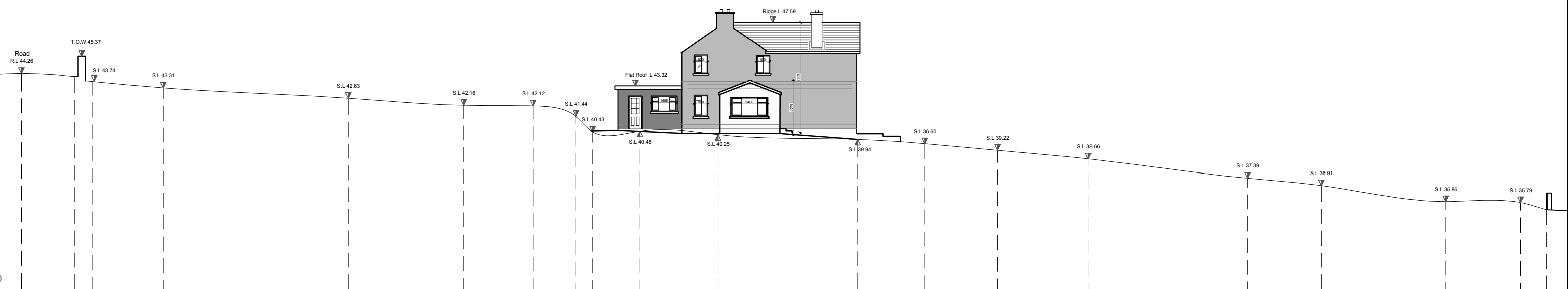
NORTH SOUTH CROSS SECTION DD EXISTING SCALE 1:250 A3
