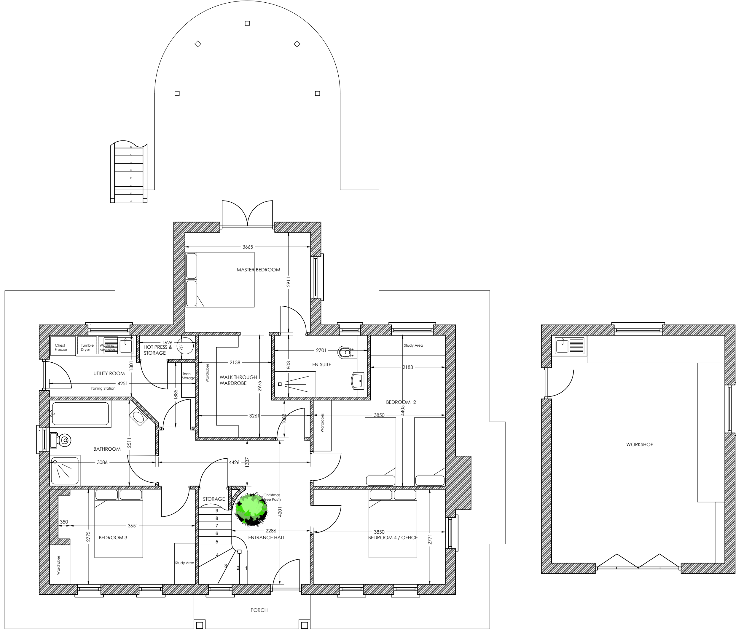
GROUND FLOOR LAY-OUT
