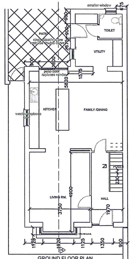
GROUND FLOOR PLAN TOTAL FLOOR AREA 129 sq.mts.
