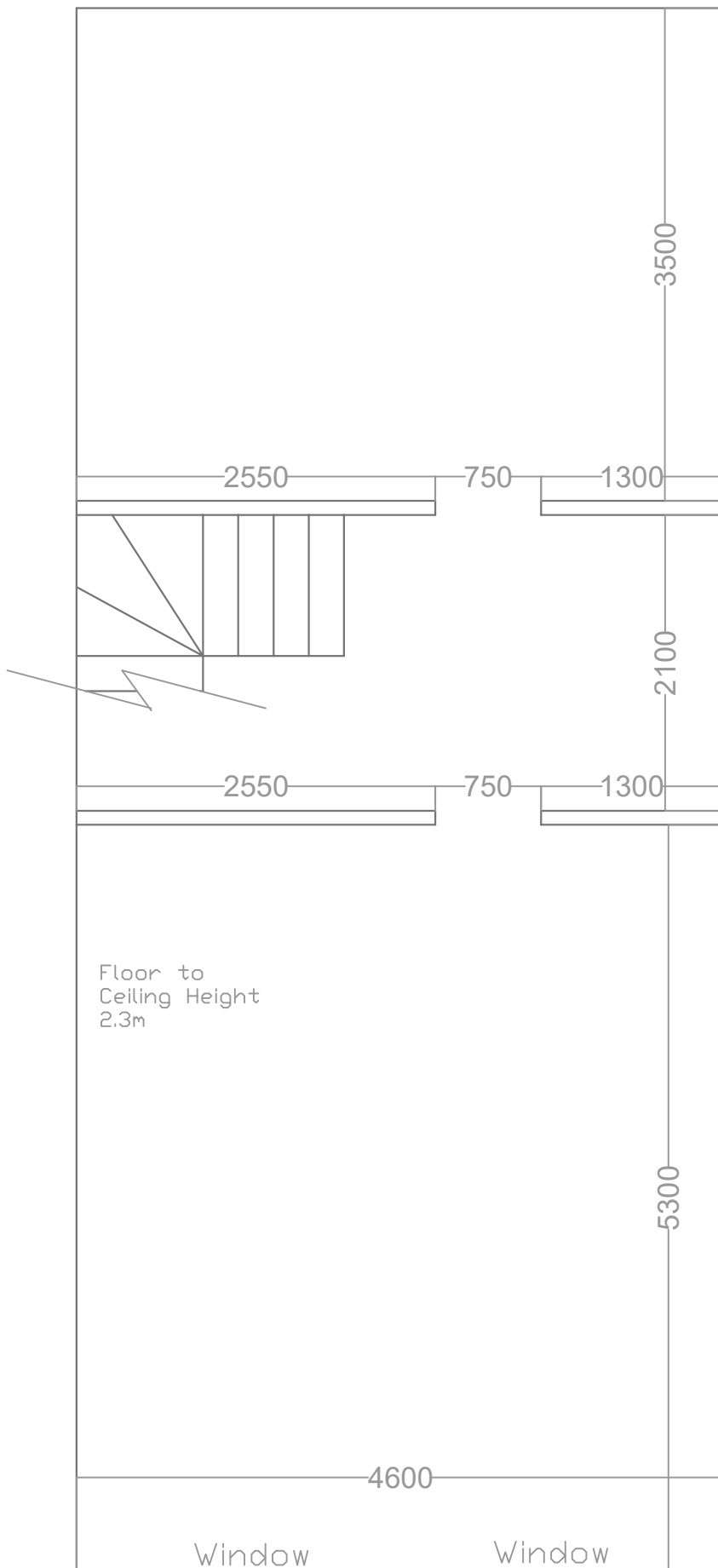
44 North Main Street Second Floor Plan
